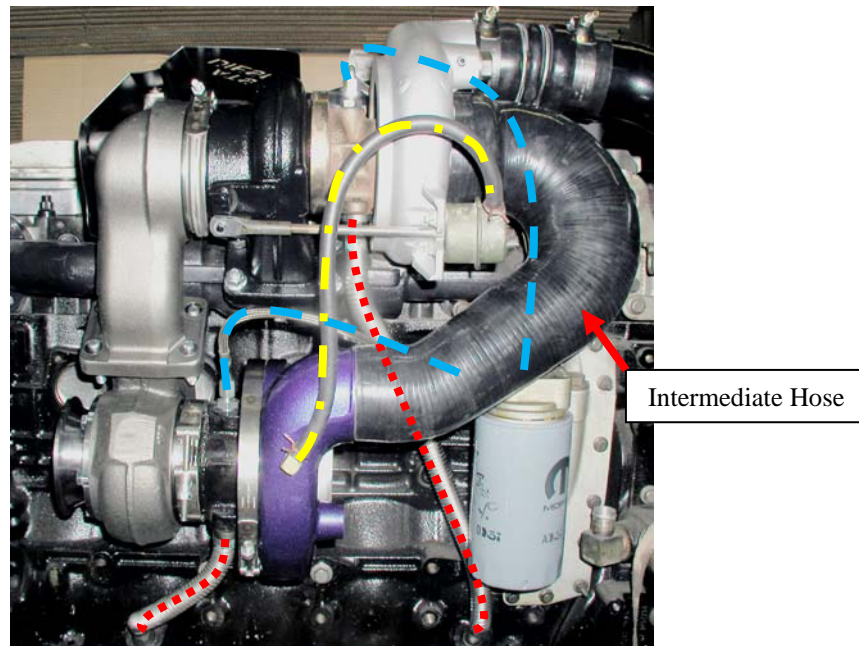
Figure 3: Line and Drain Tube Routing
