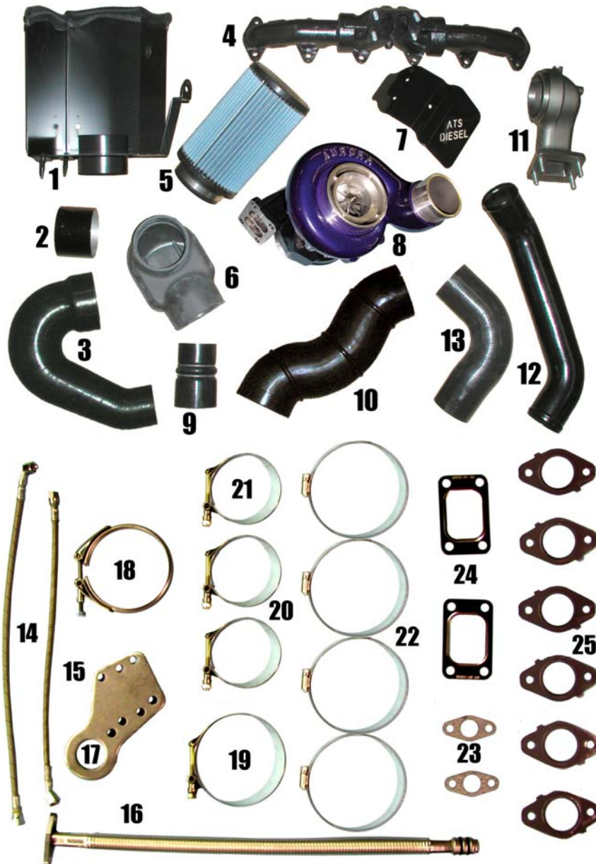
Figure 1: Aurora Plus - 4000 Kit Contents
